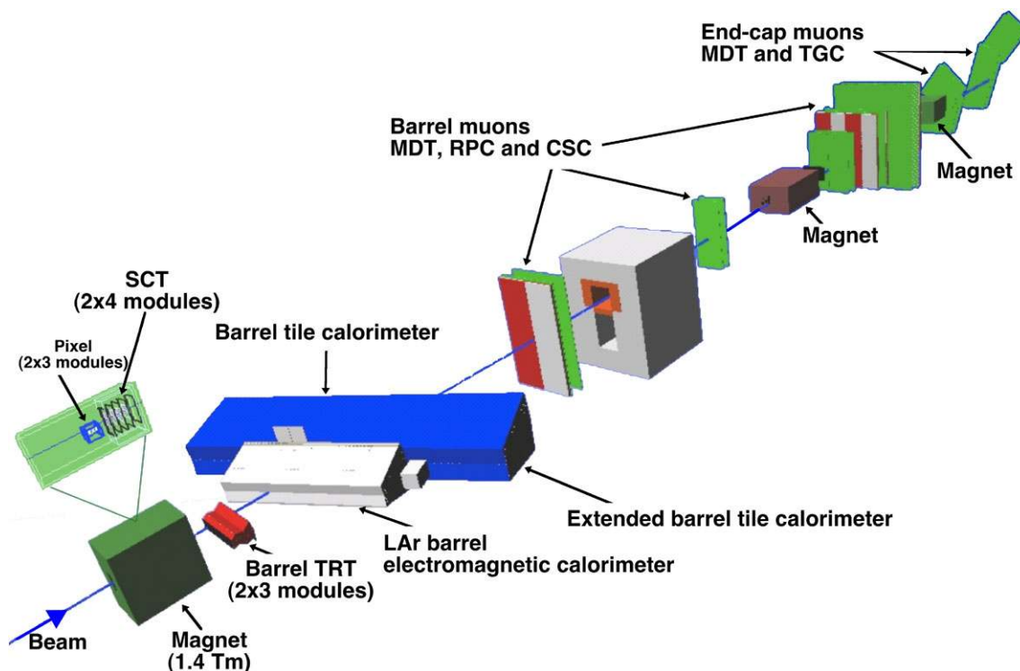
Fig. 4 Combined test beam setup from 2004
