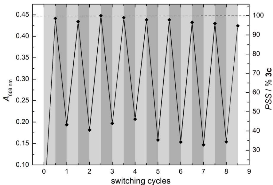
Figure 2. Composition of the photostationary state (PSS, right) as measured by the long-wavelength absorption maximum of 3c at 608 nm during alternating switching cycles consisting of ring-closure ( \lambda(\text{irr}) = 405 \text{ nm} , t = 20 \text{ min} , light grey areas) and ring-opening ( \lambda(\text{irr}) > 500 \text{ nm} , t = 100 \text{ min} , grey areas) of a 2 \times 10^{-5} \text{ M} degassed acetonitrile solution with a 1000 W high-pressure Xe lamp. The maximum for pure 3c is indicated by the dashed line.
