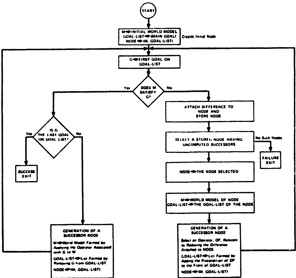
FIG. 2. Flow chart for STRIPS.
