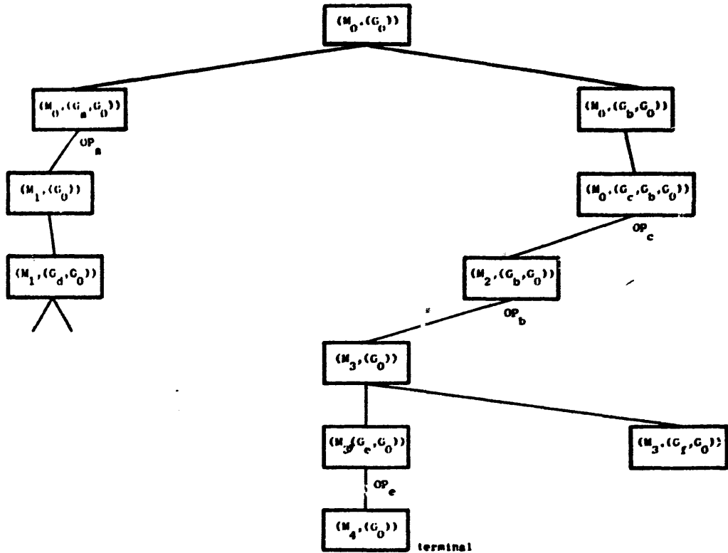
FIG. 1. A typical STRIPS search tree.
