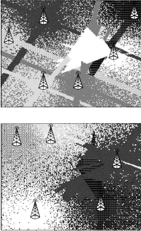
Fig. 2: Calculated mmWave BS associations with real building locations [58]. The shaded regions correspond to association with the BS centered at that shade. Blocking, LOS vs. non-LOS propagation, and beam directionality render our usual notion of cell boundaries obsolete.
