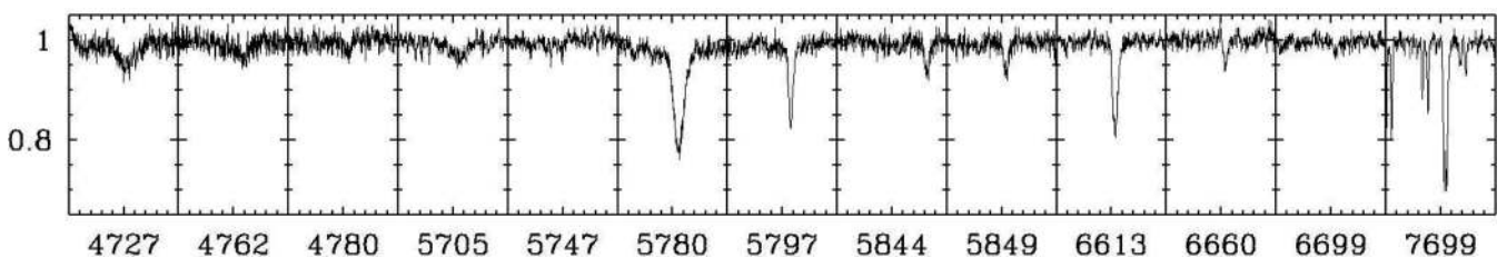
Figure 7. Preliminary data on DIBs and on the \text{K I} interstellar atomic line at 7699\text{ \AA} as observed by GALAH. Spectrum of TYC 4011-102-1, a hot star with strong interstellar absorptions close to the Galactic plane, is shown. Each 20\text{ \AA} wide panel is centred on the DIB wavelength as listed in Jenniskens & Desert (1994). Plotted wavelengths are heliocentric. Right-most panel identifies two interstellar clouds for \text{K I} at different velocities. For a majority of GALAH objects which lie away from the Galactic plane such complications are rare (but can be detected).
