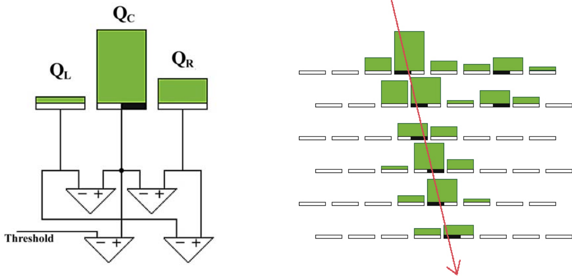
Figure 7.57: Left panel: a simplified schematic of the idea behind the comparator network. For each group of 3 adjacent strips, comparators compare the central strip signal Q_c with a threshold and with the central-to-left Q_c - Q_l , central-to-right Q_c - Q_r , and right-to-left Q_r - Q_l strip signal differences. If Q_c > \text{threshold} , Q_c - Q_l > 0 , Q_c - Q_r > 0 , and Q_r - Q_l > 0 (as shown here), the hit position is somewhere within the right half of the central strip. Right panel: a cathode local charged track is a pattern of half-strip hits consistent with a muon track.
