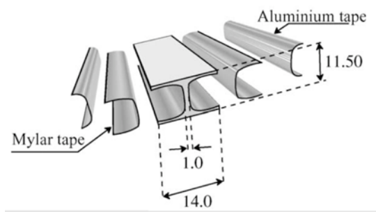
Figure 7.6: Exploded view of the cathode electrodes, glued on the I-beams.
