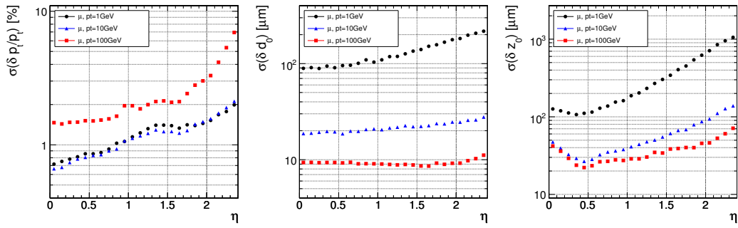
Figure 3.4: Resolution of several track parameters for single muons with transverse momenta of 1, 10 and 100 GeV: transverse momentum (left panel), transverse impact parameter (middle panel), and longitudinal impact parameter (right panel).
