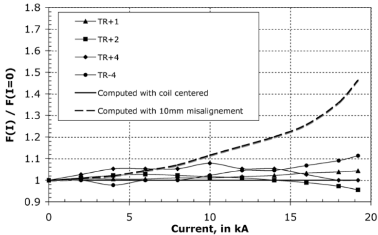
Figure 2.15: Force increase on several radial tie rods; the average force at zero current is 15 tons.
