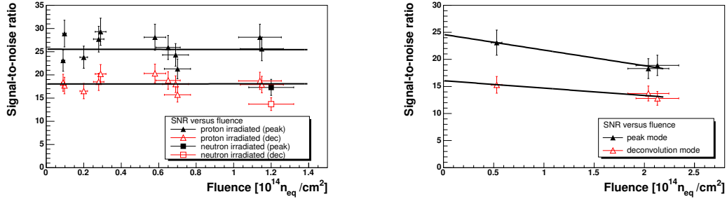
Figure 3.41: Signal-to-noise ratio versus fluence for modules with 500\ \mu\text{m} (left panel) and 320\ \mu\text{m} thick sensors (right panel) in peak (filled symbols) and deconvolution mode (open symbols).
