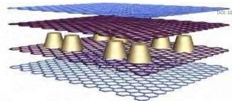
Fig. 32 Active plasmonic structure: Au dots sandwiched between SLG/h-BN layers.
