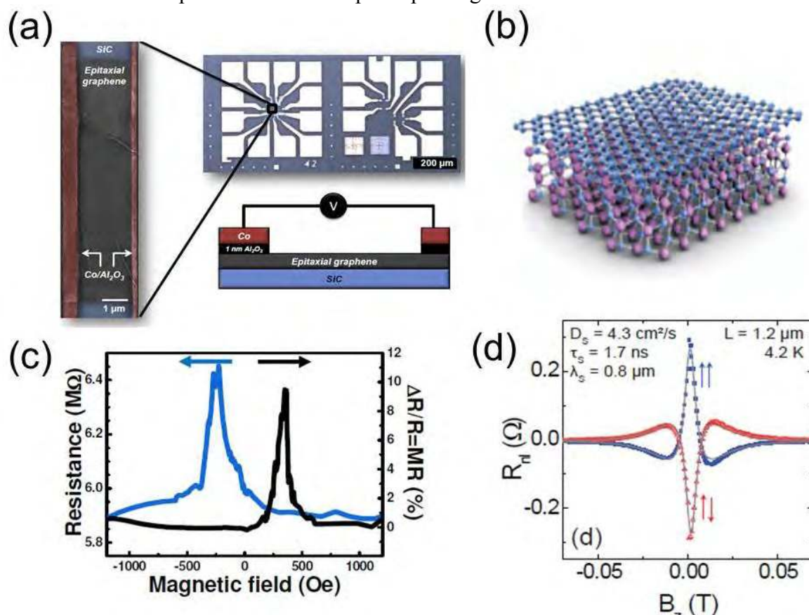
Fig. 71 (a) Typical two-terminal local spin valve device. The width of graphene channel on SiC is 10\mu\text{m} , and the distance between the two \text{Al}_2\text{O}_3/\text{Co} electrodes is L=2\mu\text{m} . The optical image shows the entire structure, including contact pads. (b) Atomic arrangement of SLG on SiC. (c) Large local resistance spin signals measured at 4K. (d) Oscillating and decaying device non-local resistance as a function of the applied magnetic field (Hanle measurement). Adapted from Refs.[223, 1300].
