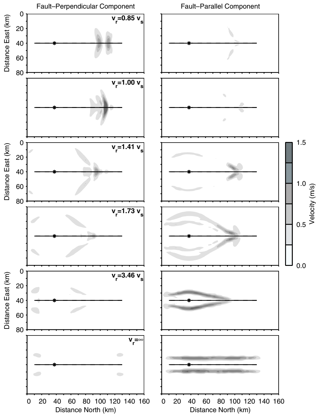
Figure 5. Snapshots of the fault-perpendicular and fault-parallel components of the velocity on the ground surface. The solid line delineates the fault trace, and the asterisk identifies the epicenter. The snapshots for each rupture speed correspond to the time at which the rupture at the surface has propagated approximately 65 km down the fault, except for the case of an infinite rupture speed for which the snapshot is taken at 6.0 sec after the initiation of rupture. As the rupture speed increases, the amplitude of the shear wave radiated along the strike of the fault decreases, whereas the amplitude of the shear wave radiated perpendicular to the fault increases.
