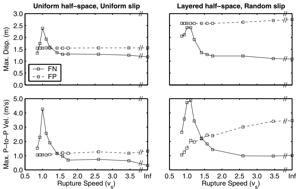
Figure 10. Overall maximum fault-parallel (FP) and fault-perpendicular (FN) displacement and peak-to-peak velocity for any point on the ground surface as a function of rupture speed. The left column shows the values for the uniform half-space with uniform slip, and the right column shows the values for the layered half-space with random slip. The maximum motions rotate from predominantly fault perpendicular to fault parallel as the rupture speed increases to intersonic and supersonic speeds. The two models display very similar behavior, although the random spatial variation in slip in the layered half-space results in a much larger maximum fault-parallel displacement.
