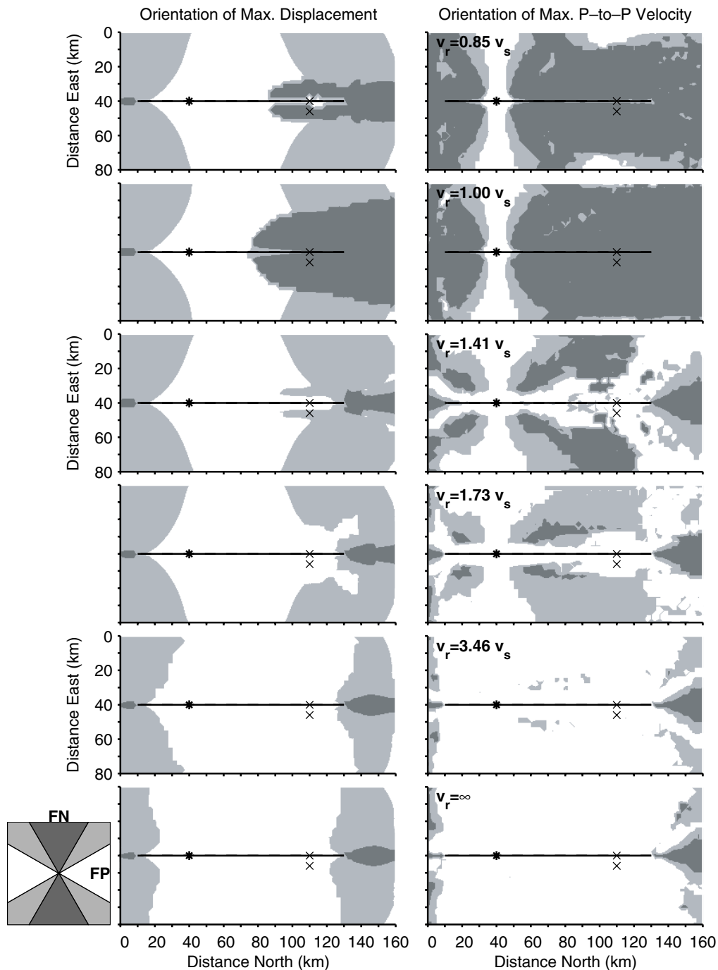
Figure 7. Orientation of the maximum horizontal displacements and peak-to-peak velocities for six rupture speeds. The solid line delineates the fault trace, and the asterisk identifies the epicenter. The maximum motion rotates from predominantly fault-perpendicular (FN) to fault-parallel (FP) orientations as the rupture propagation moves from subshear speeds to supersonic speeds. Figure 8 shows the velocity time histories for the sites designated by \times .
