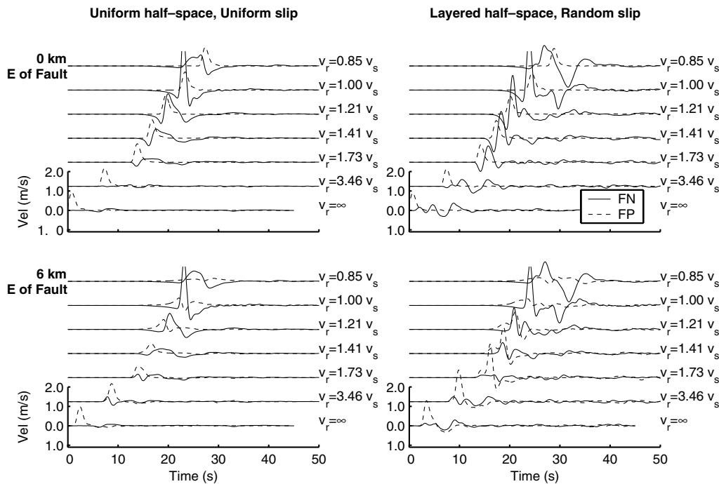
Figure 8. Fault-parallel (FP) and fault-perpendicular (FN) velocity time histories at two sites (see Figs. 1 and 7) for seven different rupture speeds in the uniform half-space with uniform slip ( left ) and the layered half-space with random slip ( right ). The sites lie 0 km or 6 km east of the fault near the north end (100 km along strike). These time histories illustrate that for sites near the rupture, at subshear propagation speeds the energy arrives with strong fault-perpendicular motion. As the rupture speed increases, the energy arrives with increasingly earlier and larger fault-parallel motion, whereas the fault-perpendicular motion decreases.
