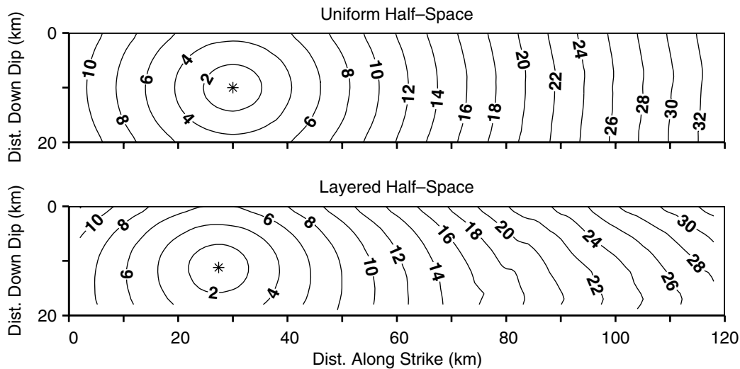
Figure 4. Progression of the leading edge of rupture as shown by contours of slip starting time (in seconds) for the uniform half-space (top) and the layered half-space (bottom) for a rupture propagating at 85% of the local shear-wave speed in the mode-II direction and 20% slower in the mode-III direction. In both cases, the rupture propagates predominantly in the mode-II (horizontal) direction. In the layered half-space the rupture propagates faster at depth and drives the rupture along the surface. The hypocenters indicated by the stars sit 30.0 km and 27.2 km along strike at depths of 10.0 km and 11.2 km, respectively. Roughness in the contours for the layered half-space arise from generating contours from an unstructured finite-element mesh with significant variations in element size.
