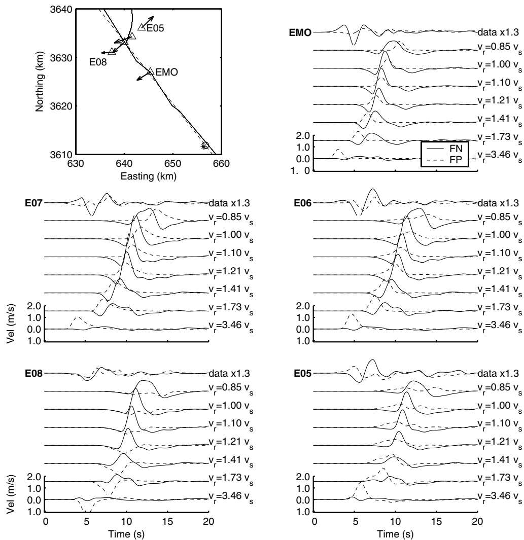
Figure 12. Orientation of the peak velocity (upper left) and comparison of velocity waveforms from the 1979 Imperial Valley earthquake for four stations in the El Centro strong-motion array (stations E05 to E08) and station EMO. The triangles identify the station locations, and the vectors show the amplitude and orientation of the maximum velocity. The solid line indicates the fault trace, and the asterisk identifies the epicenter. The dashed line and open circle show the comparable geometry for the simulations. The maximum velocities are generally aligned with the fault-perpendicular direction, and the stations generally experience significant fault-perpendicular (FN) motion prior to fault-parallel (FP) motion, implying most of the energy was generated while the rupture propagated slower than the shear-wave speed.
