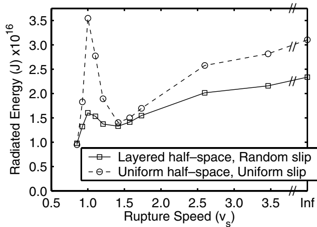
Figure 11. Far-field radiated energy as a function of rupture speed for both the uniform half-space with uniform slip and the layered half-space with random slip. The maximum in the shear-wave radiation pattern along the strike of the fault results in a significant increase in the radiated energy for rupture speeds approaching the shear-wave speed. In the layered half-space, the depth variation in the shear-wave speed limits the amplitude of the peak in radiated energy for a rupture propagating at the shear-wave speed. The local minimum for intersonic rupture occurs at the Eshelby speed. Approaching supersonic speeds, the radiated energy increases because of effective reinforcement of the shear waves radiated perpendicular to the fault.
