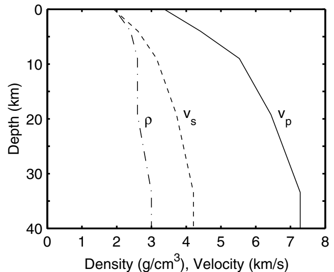
Figure 2. Dilatational-wave speed ( v_p ), shear-wave speed ( v_s ), and mass density ( \rho ) as a function of depth for the layered half-space.
