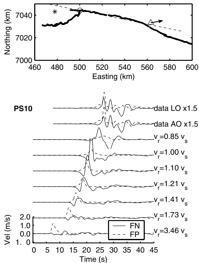
Figure 13. Orientation of the peak velocity (top) and comparison of velocity waveforms from the 2002 Denali fault earthquake for the pump station 10 record. The triangles identify the station location, and the vector shows the amplitude and orientation of the maximum velocity. The thick solid line indicates the fault trace, and the asterisk identifies the epicenter. The dashed line and open circle show the comparable geometry for the simulations. The data are shown with fault-parallel (FP) and fault-perpendicular (FN) components relative to the local fault orientation (LO) and the average fault orientation (AO). An 8-sec time delay applied to the data to allow a more direct comparison with the simulations. The orientation of the peak velocity and the velocity waveforms fit the pattern for rupture above the shear-wave speed.
