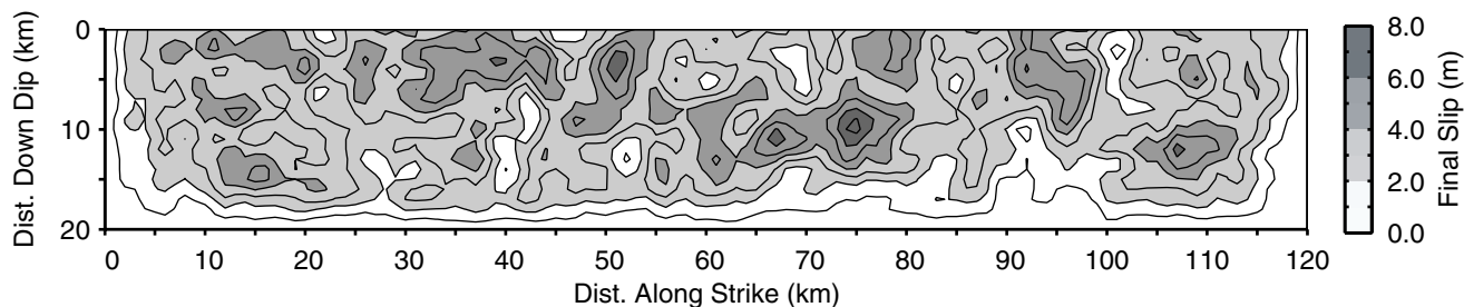
Figure 3. Distribution of final slip created from low-pass filtering a random distribution. The average slip is 2.9 m, with a maximum value of 7.1 m, yielding a moment magnitude of 7.4.
