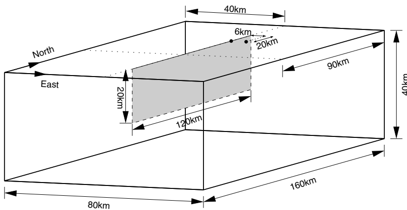
Figure 1. Geometry of the simulation domain. The center of the fault lies 10 km south of the center of the domain. We examine shear-wave polarization at the sites denoted by the dots, which sit at distances of 0 km and 6 km from the fault trace near the northern end of the rupture.
