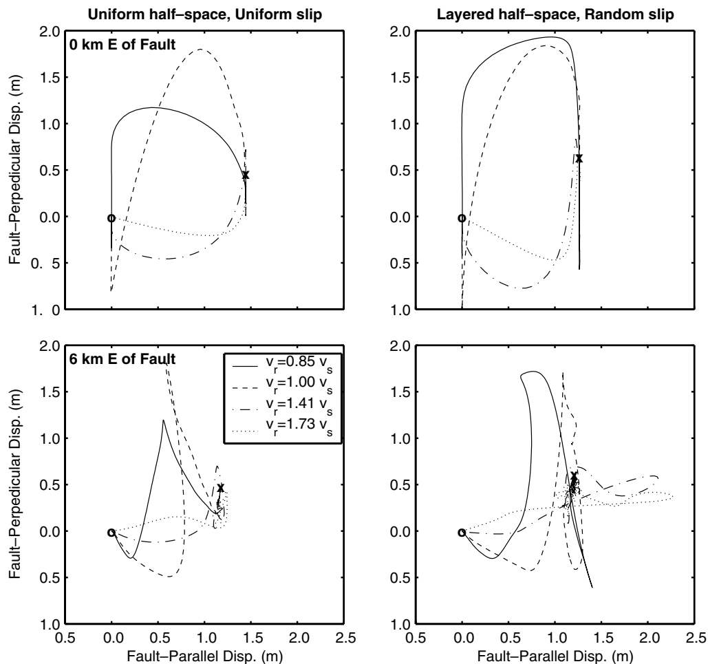
Figure 9. Displacement trajectories at two sites (same sites as in Fig. 8) for four different rupture speeds in the uniform half-space with uniform slip (left) and the layered half-space with random slip (right). The trajectories begin at the origin (denoted by circles) and end at the Xs. The trajectories demonstrate that sites very close to the fault experience fault-parallel motion after fault-perpendicular motion for subshear rupture, whereas for supershear rupture, the sites experience fault-parallel motion before significant fault-perpendicular motion. Beginning at distances of around 6 km from the fault, the effects of the dilatational wave become significant, and this feature disappears.
