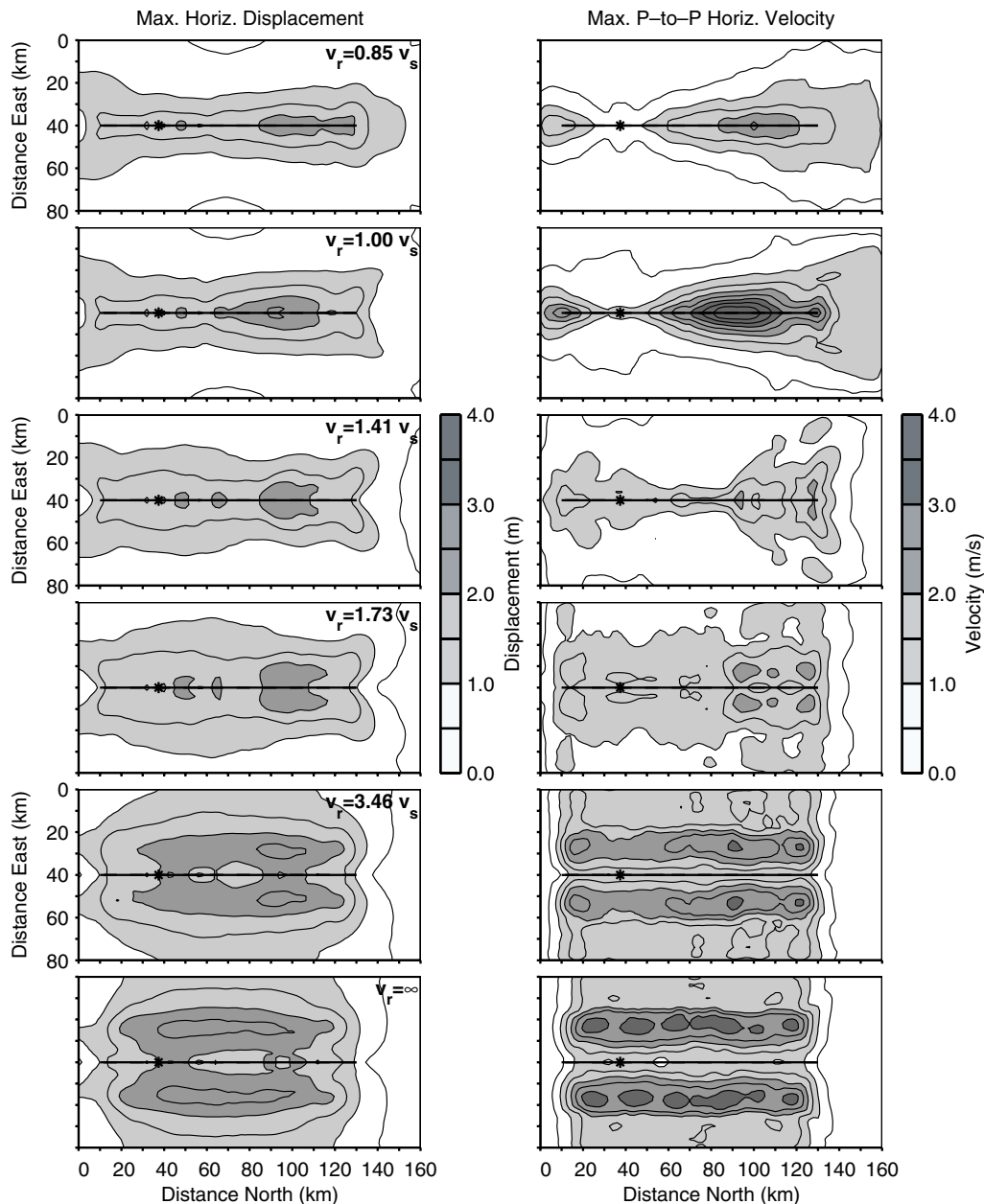
Figure 6. Maximum horizontal displacements and peak-to-peak velocities on the ground surface for six rupture speeds. The solid line delineates the fault trace, and the asterisk identifies the epicenter. Increasing the rupture propagation from subshear speeds to supersonic speeds shifts the distribution of shaking from a tear-drop shape associated with larger amplitudes along the strike of the fault away from the epicenter to an elliptical shape associated with very large amplitudes along the entire strike of the fault at distances out to one fault width from the fault trace.
