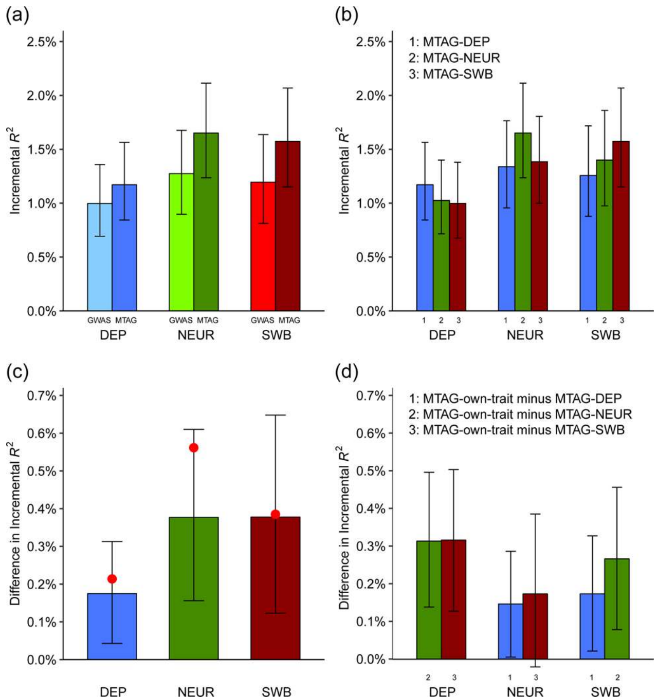
Fig. 6. Predictive power of GWAS- and MTAG-based polygenic scores
