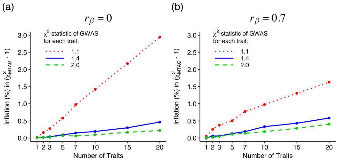
Fig. 1. Bias in standard errors from ignoring sampling variation in \hat{\Sigma} and \hat{\Omega}
