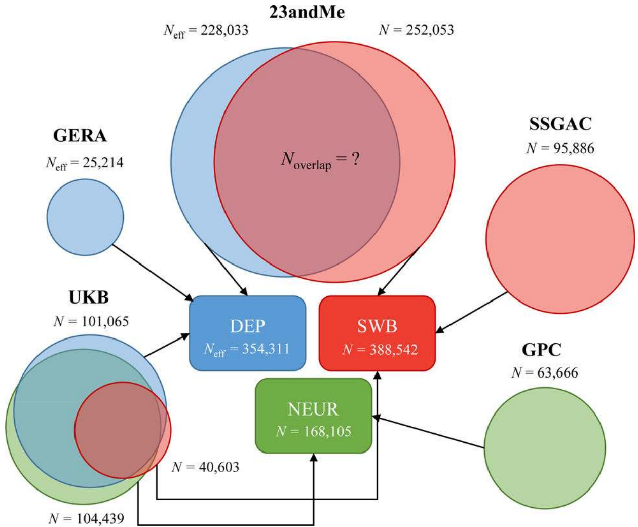
Fig. 3. Cohorts included in GWAS meta-analyses for DEP, NEUR, and SWB
