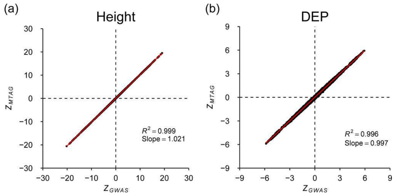
Fig. 2. Evaluation of MTAG's standard errors when there is sample overlap
