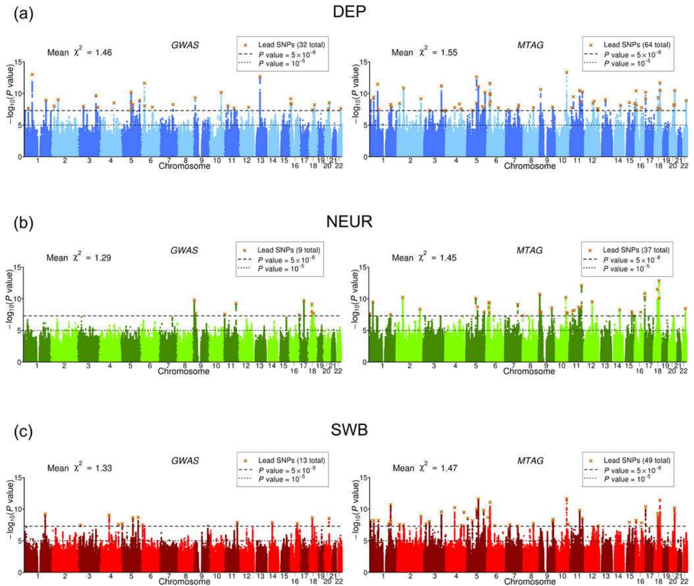
Fig. 4. Manhattan plots of GWAS and MTAG results
