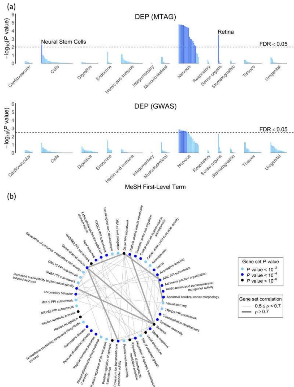
Fig. 7. Biological annotation for DEP using the bioinformatics tool DEPICT
