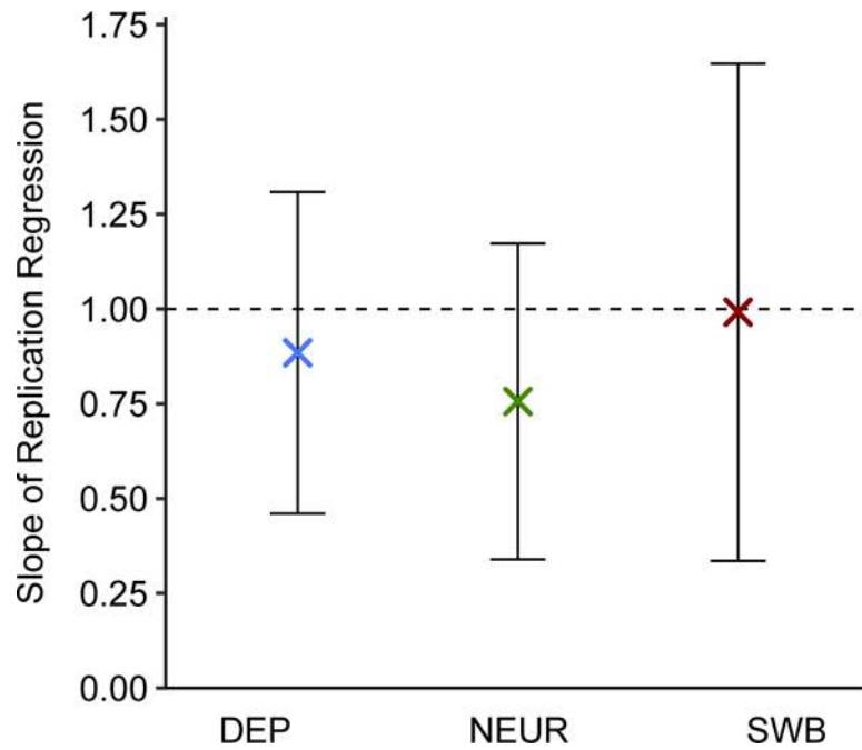
Fig. 5. Regression-based test of replicability of MTAG-identified loci
