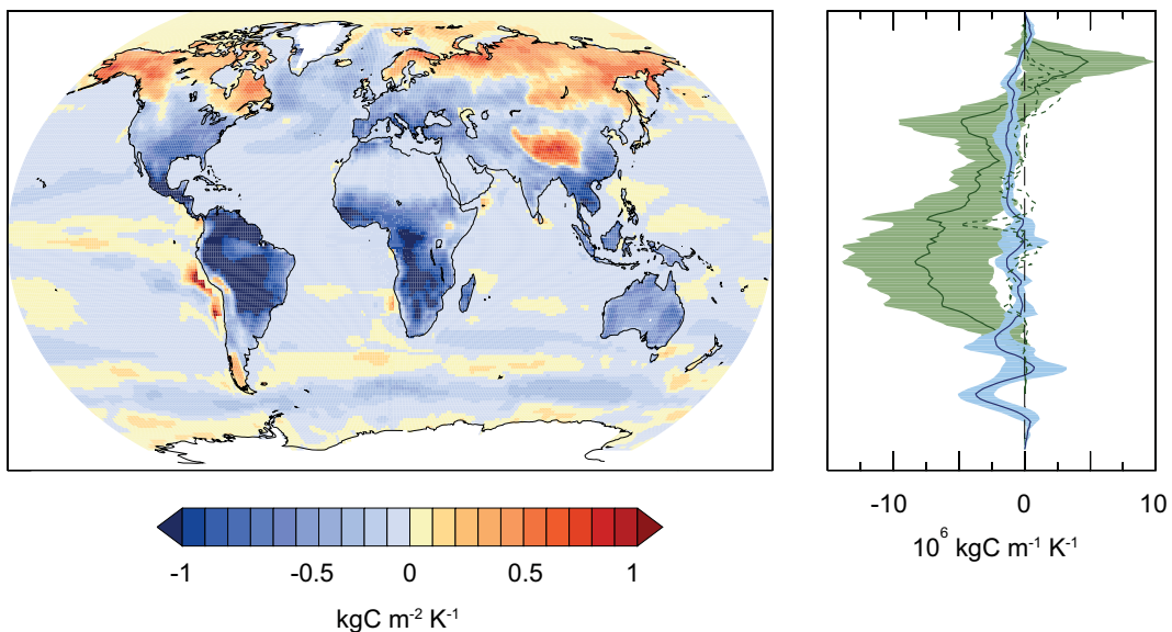
Figure 6.22: The spatial distributions of multi model-mean land and ocean \beta and \gamma for 7 CMIP5 models using the concentration-driven idealised 1% per year CO 2 simulations. For land and ocean, \beta and \gamma are defined from changes in terrestrial carbon storage and changes in air-sea integrated fluxes respectively, from 1xCO 2 to 4xCO 2 , relative to global (not local) CO 2 and temperature change. In the zonal mean plots, the solid lines show the multi-model mean and shaded areas denote \pm 1 standard deviation. Models used are: BCC-CSM1-1, CanESM2, CESM1-BGC, HadGEM2-ES, IPSL-CM5A-LR, MPI-ESM-LR, NorESM1-ME. The dashed lines show the models that include a land carbon component with an explicit representation of N-cycle processes (CESM1-BGC, NorESM1-ME).
