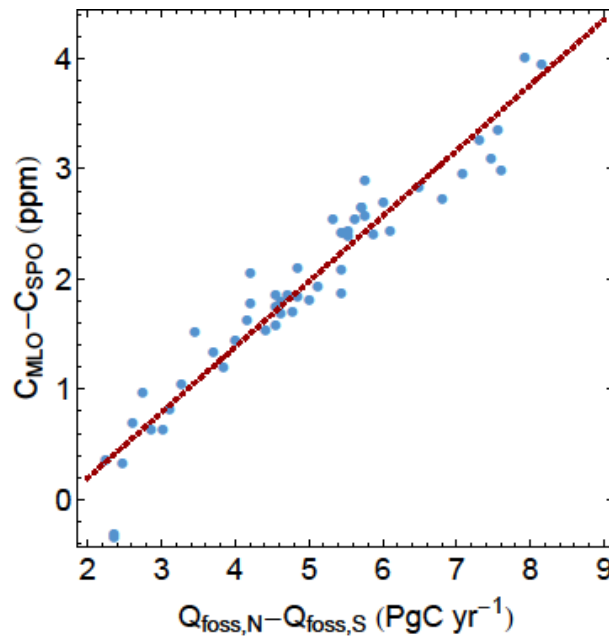
Figure 6.13: Blue points: Annually averaged \text{CO}_2 concentration difference between the station Mauna Loa in the northern hemisphere and the station South Pole in the southern hemisphere (vertical axis; Keeling et al., 2005, updated) versus the difference in fossil fuel combustion \text{CO}_2 emissions between the hemispheres (Boden et al., 2011). Dark red dashed line: regression line fitted to the data points.
