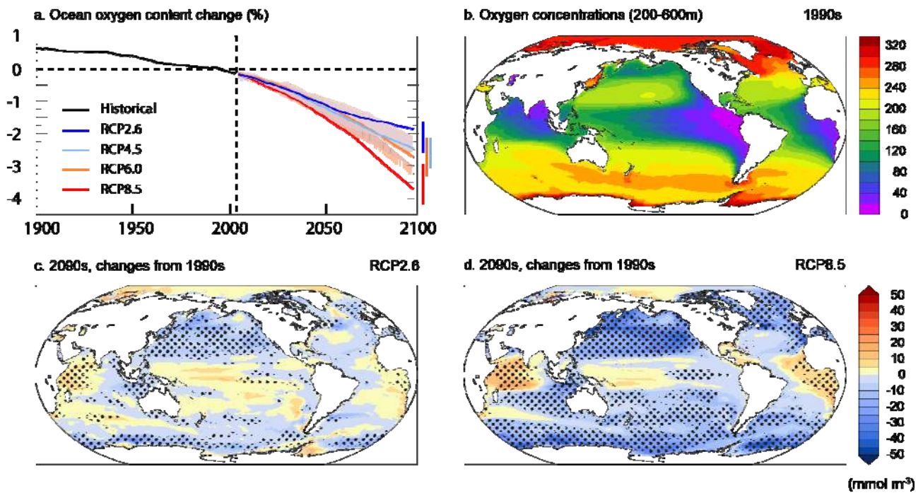
Figure 6.30: (a) Simulated changes in dissolved \text{O}_2 (mean and model range as shading) relative to 1990s for RCP2.6, RCP4.5, RCP6.0 and RCP8.5. (b) Multi-model mean dissolved \text{O}_2 ( \mu\text{mol m}^{-3} ) in the main thermocline (200 to 600m depth average) for the 1990s, and changes in 2090s relative to 1990s for RCP2.6 (c) and RCP8.5 (d). To indicate consistency in the sign of change, regions are stippled where at least 80% of models agree on the sign of the mean change. These diagnostics are detailed in Cocco et al. (2013) in a previous model intercomparison using the SRES-A2 scenario and have been applied to CMIP5 models here. Models used: CESM1-BGC, GFDL-ESM2G, GFDL-ESM2M, HadGEM2-ES, IPSL-CM5A-LR, IPSL-CM5A-MR, MPI-ESM-LR, MPI-ESM-MR, NorESM1.
