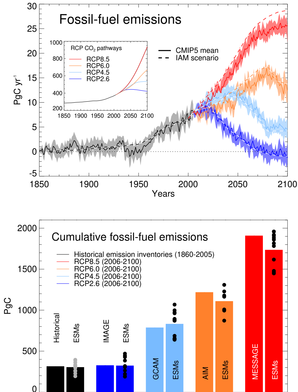
Figure 6.25: Compatible fossil fuel emissions simulated by the CMIP5 ESM models for the 4 RCP scenarios. Top: time series of compatible emission rate (PgC yr -1 ). Dashed lines represent the historical estimates and emissions calculated by the integrated assessment models (IAM) used to define the RCP scenarios, solid lines and plumes show results from CMIP5 ESMs (model mean, with 1 standard deviation shaded). Bottom: cumulative emissions for the historical period (1860–2005) and 21st century (defined in CMIP5 as 2006–2100) for historical estimates and RCP scenarios. Dots denote individual ESM results, bars show the multi-model mean. In the CMIP5 model results, total carbon in the land-atmosphere-ocean system can be tracked and changes in this total must equal fossil fuel emissions to the system (see Box 6.4). Models used: CanESM2, GFDL-ESM2G, GFDL-ESM2M, HadGEM2-CC, HadGEM2-ES, IPSL-CM5A-LR, IPSL-CM5A-MR, IPSL-CM5B-LR, MIROC-ESM-CHEM, MIROC-ESM, MPI-ESM-LR, NorESM1-ME, INMCM4, CESM1-BGC, BCC-CSM1.1. Not every model performed every scenario simulation.
