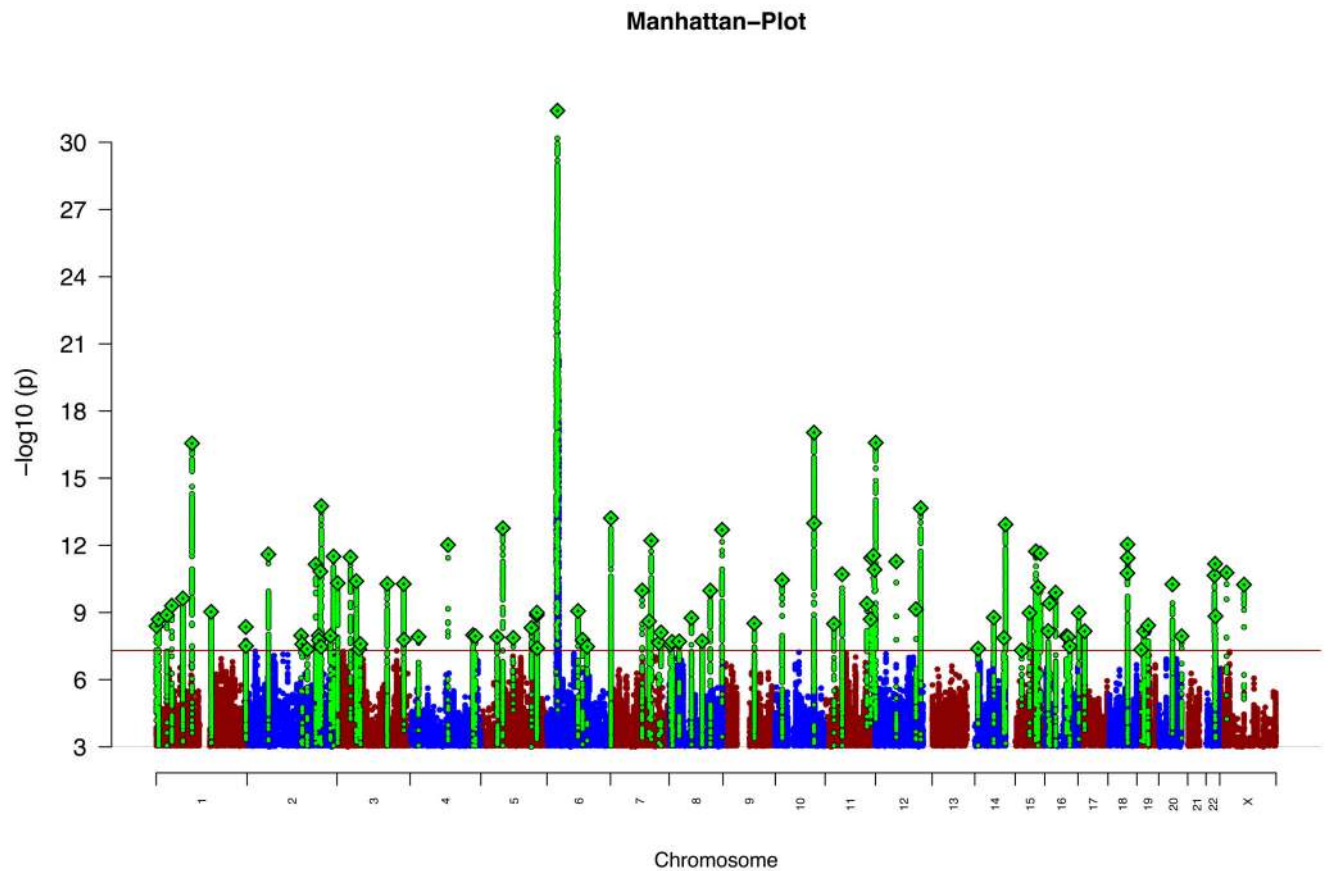
Figure 1. Manhattan plot
